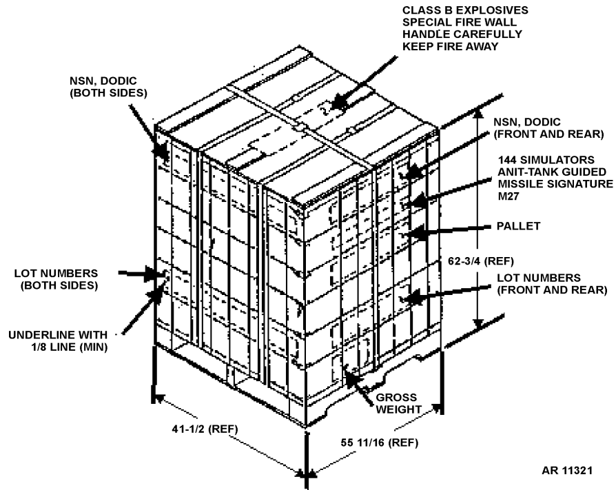
Figure 4-12. Typical Palletization.
